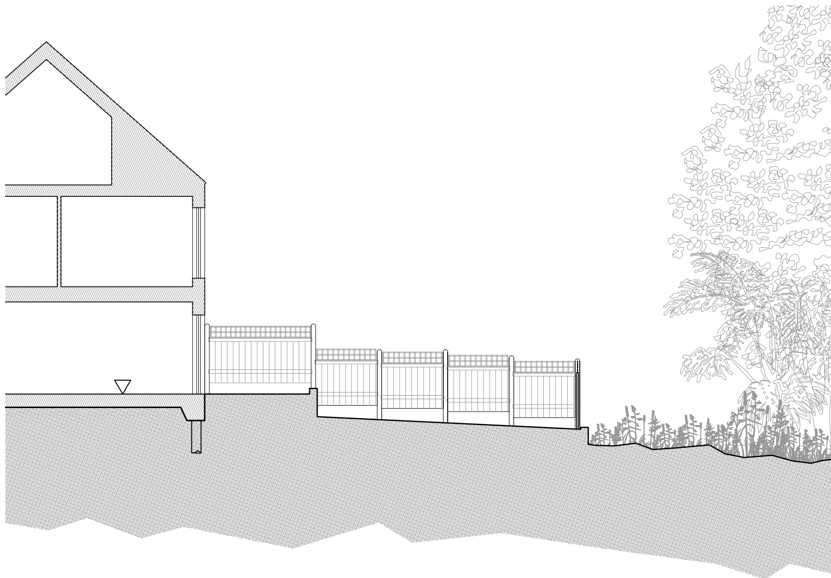
SECTION G
