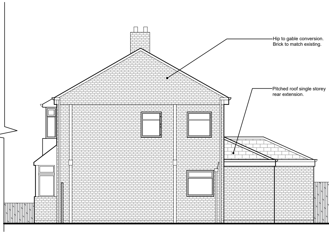
PROPOSED ELEVATION B-B SCALE 1:100
