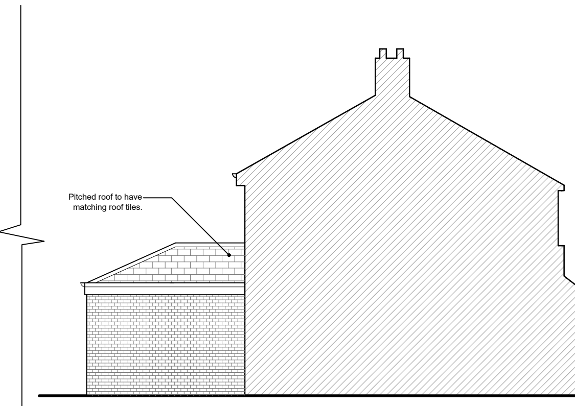
PROPOSED ELEVATION D-D SCALE 1:100
