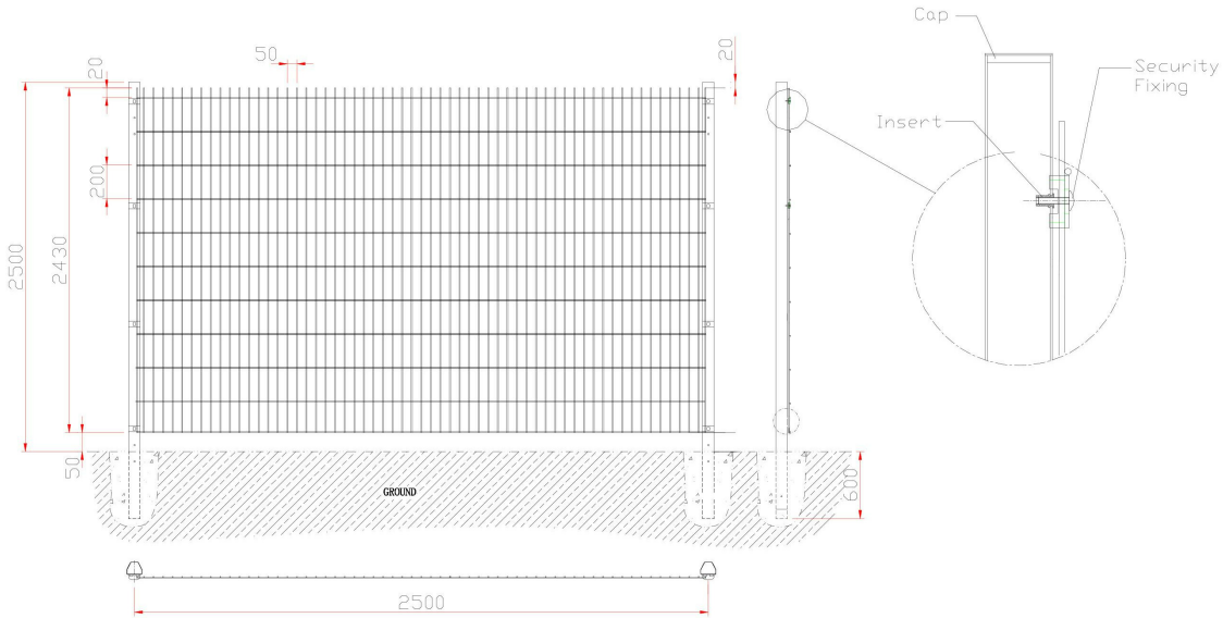
Procter Fence_Front Elevation and Section Drawings
