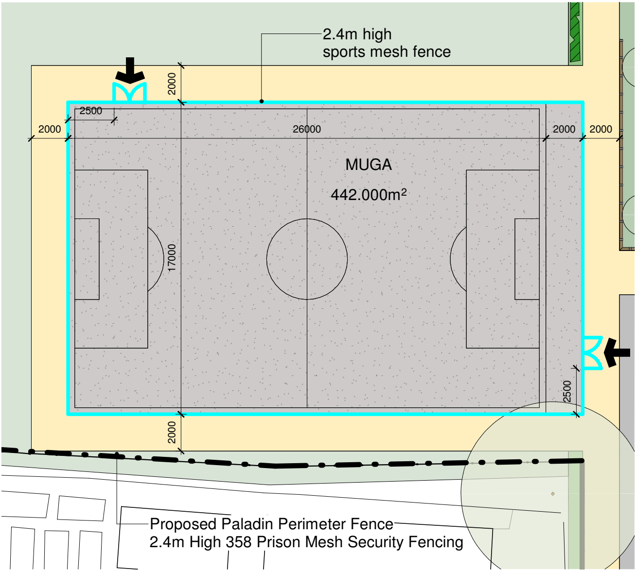
1 05-ZZ_MUGA Plan as Proposed 1 : 200
