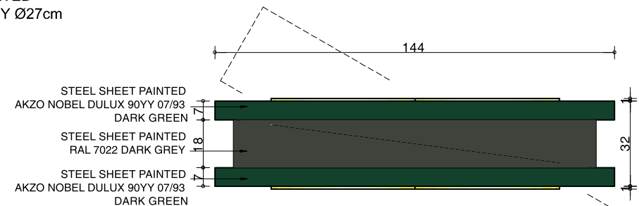
PLAN VIEW 1/20
