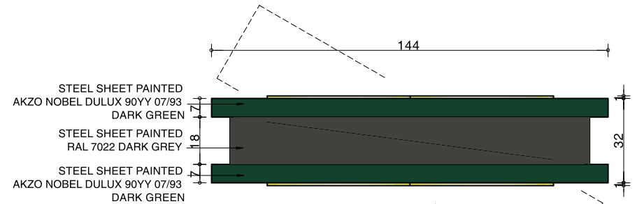
PLAN VIEW 1/20
