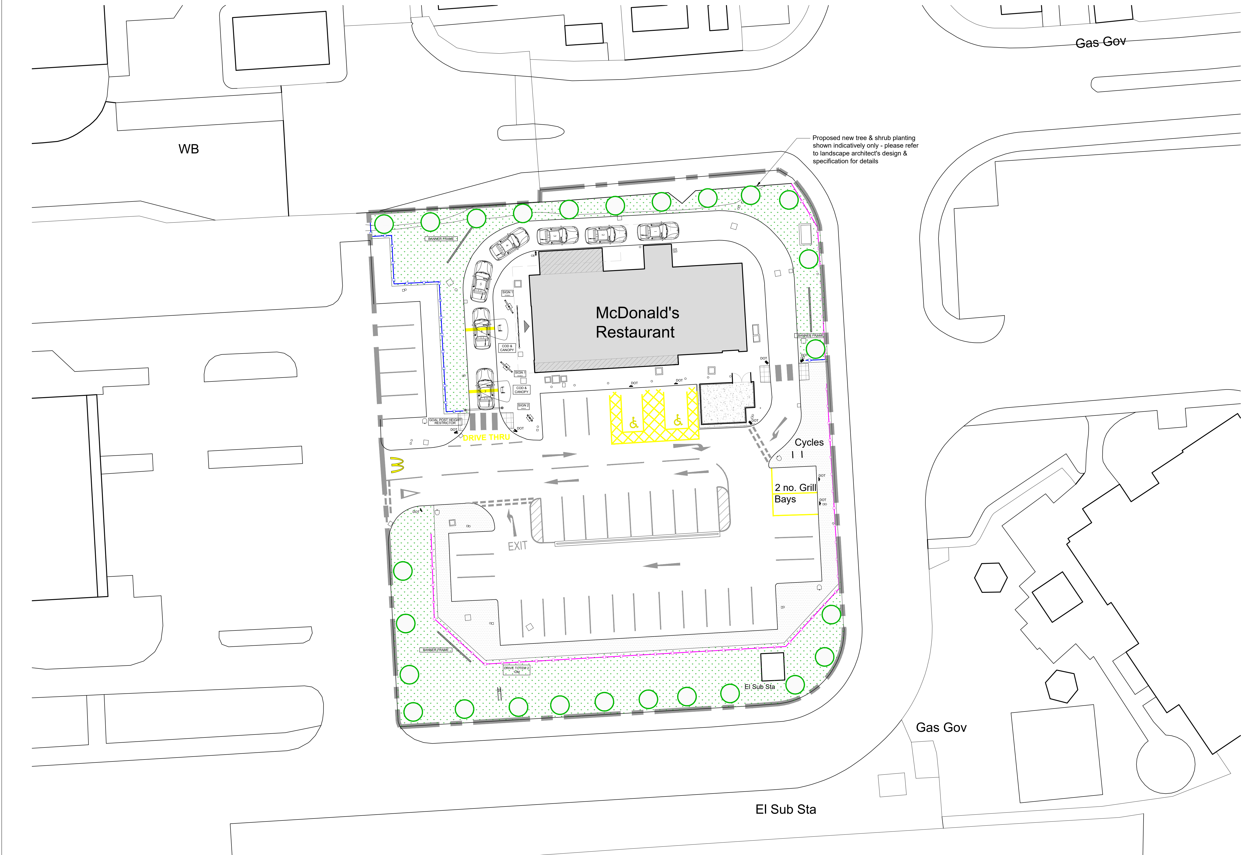
Proposed Landscape Plan
