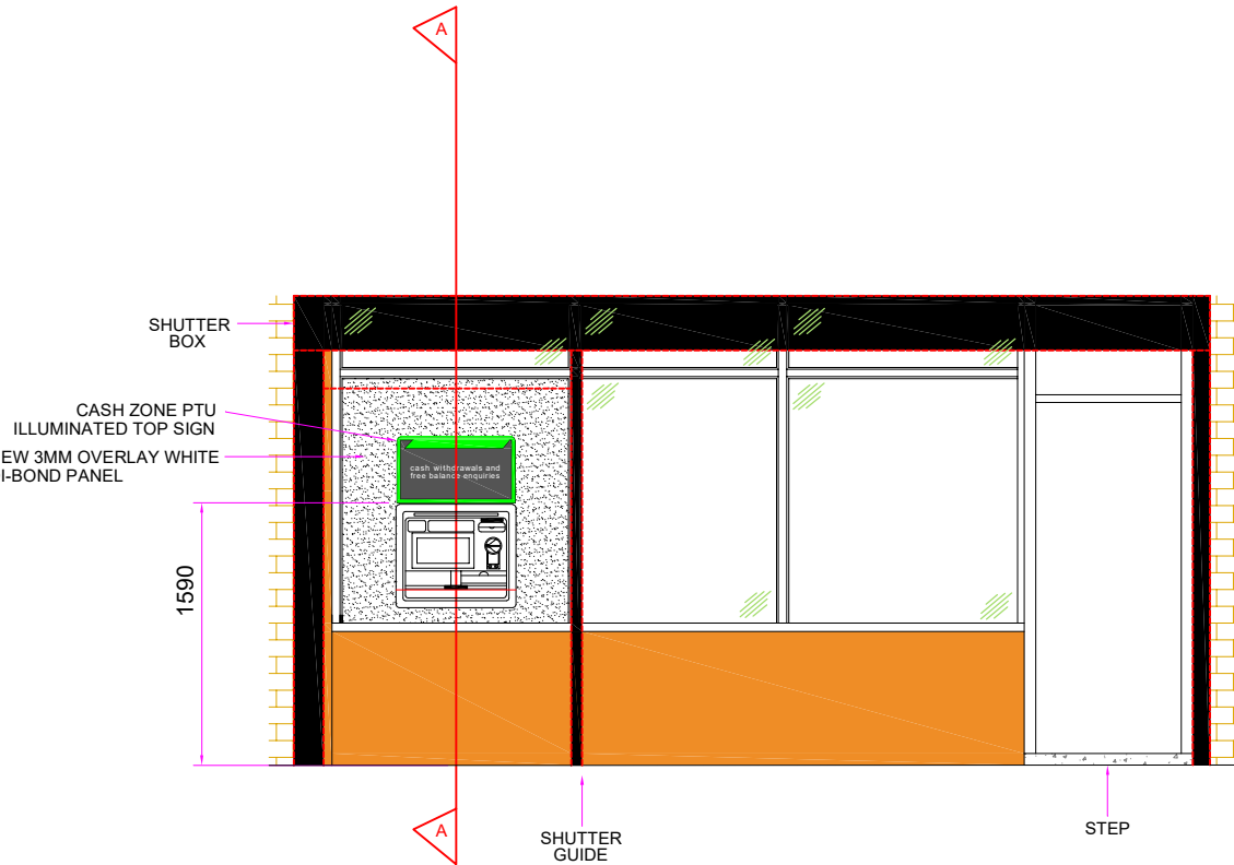
PROPOSED ELEVATION
