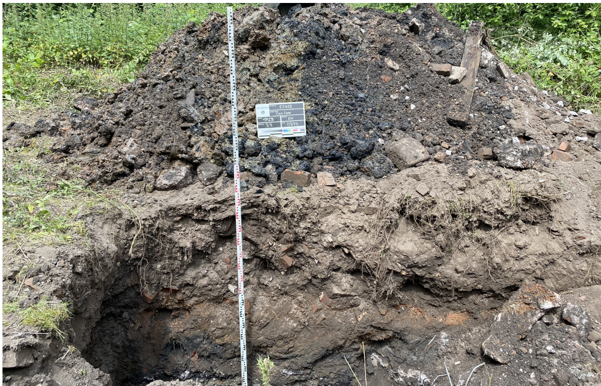
Photograph 14 – TP23 excavated to 3.8m bgl. Evidence of contamination.
