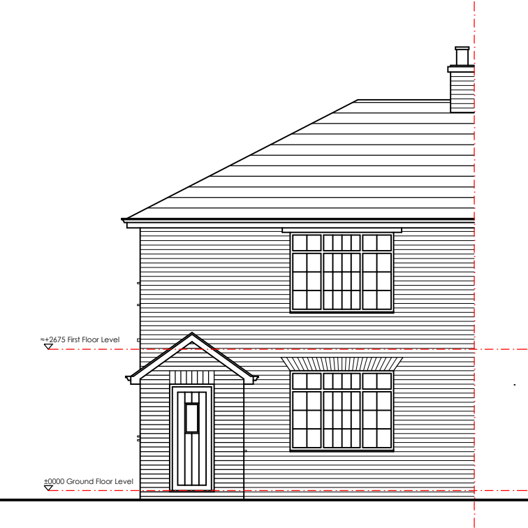
Front Elevation
