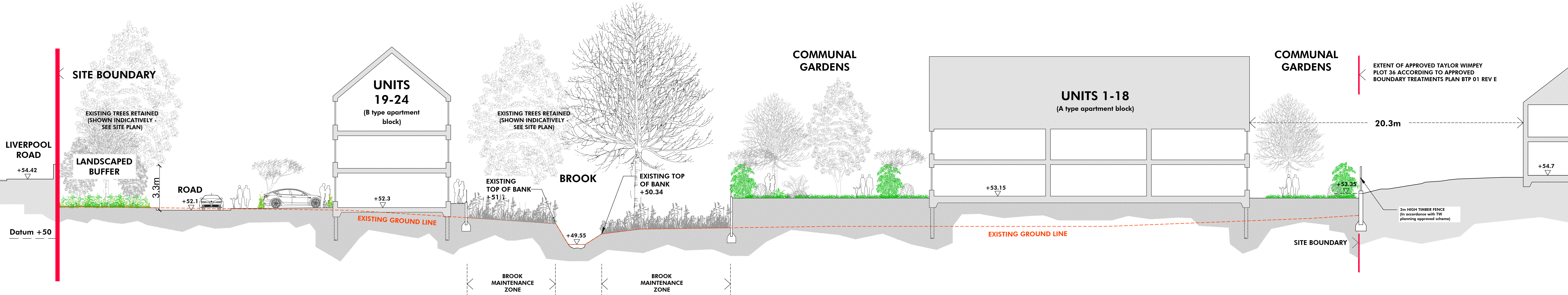
PROPOSED SECTION A-A
