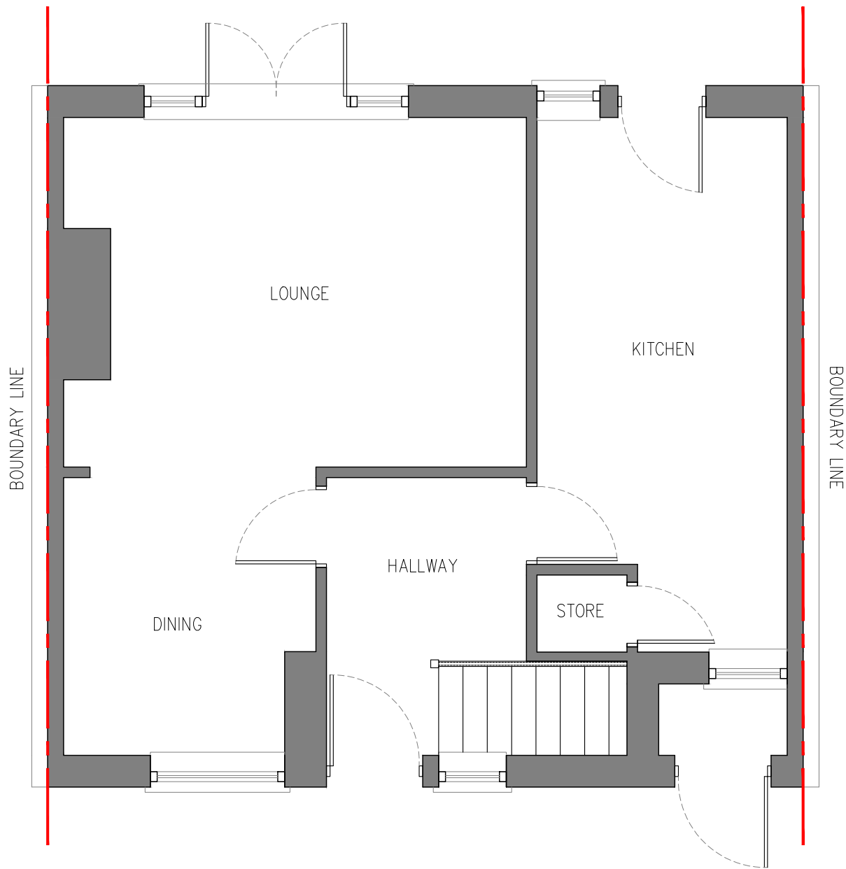
EXISTING GROUND FLOOR | SCALE 1:50
