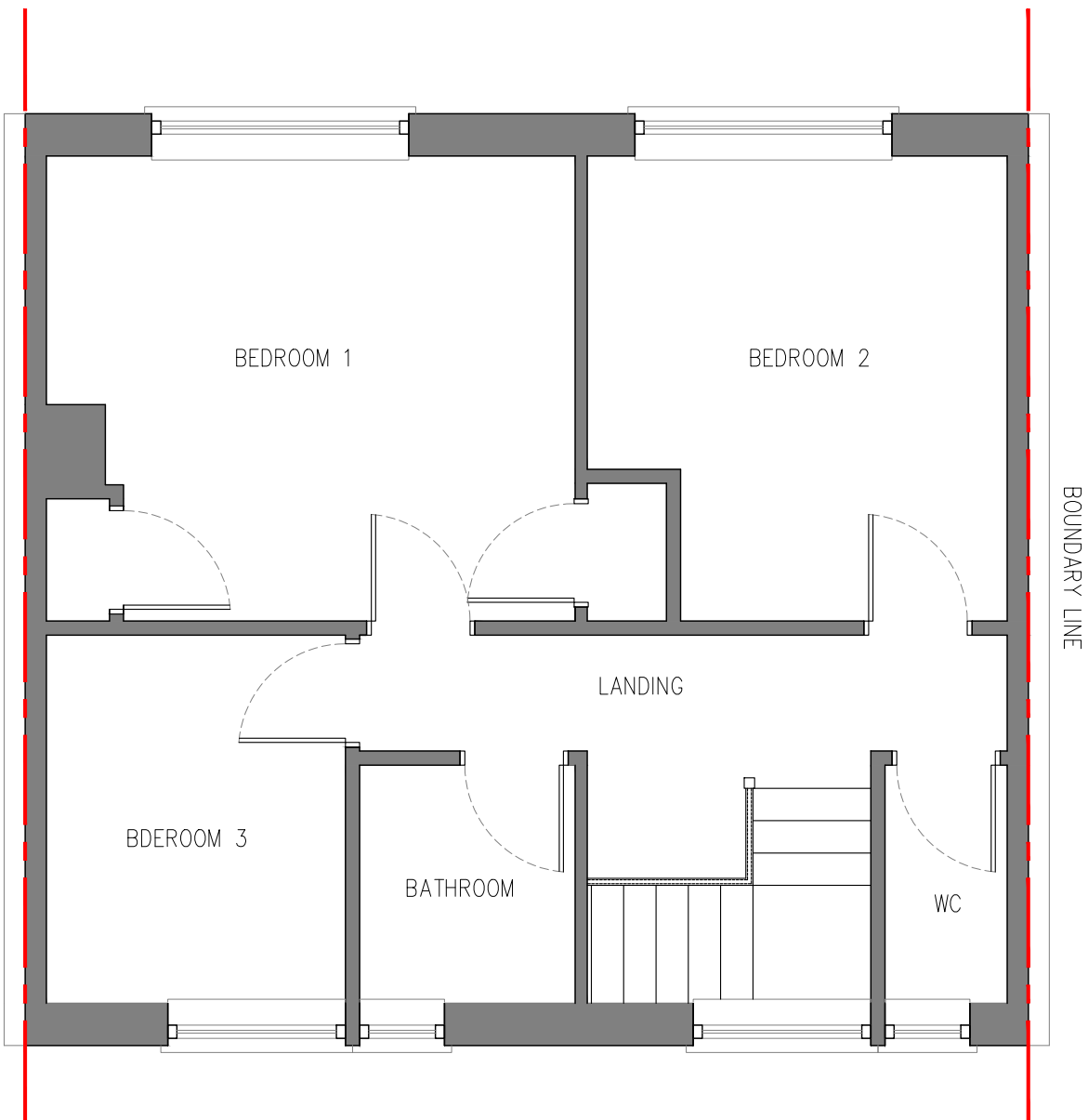
EXISTING FIRST FLOOR | SCALE 1:50
