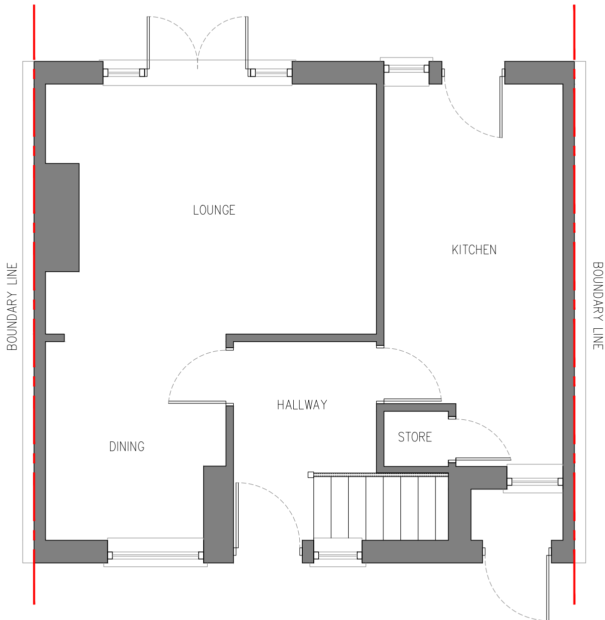
PROPOSED GROUND FLOOR | SCALE 1:50
