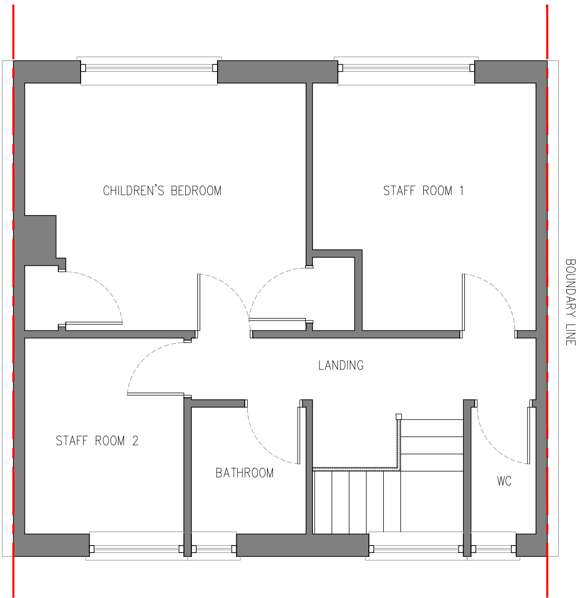
PROPOSED FIRST FLOOR | SCALE 1:50
