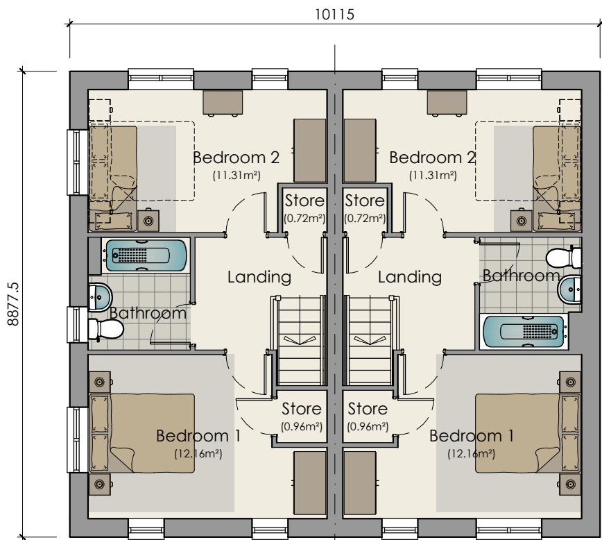
TYPE C M4(2) 2B3P 74 (OPP) FIRST FLOOR PLAN - Semi-Detached
