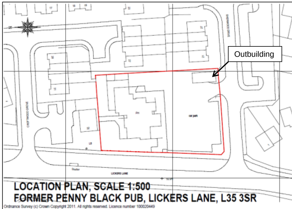
Figure 1.1 – Location plan with former pub and existing outbuilding (adapted ©Ordnance Survey 2011)
