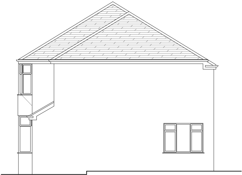
Proposed North Side Elevation 1:100
