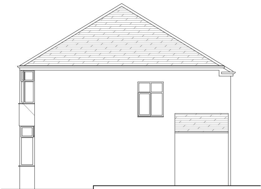
Existing North Side Elevation 1:100
