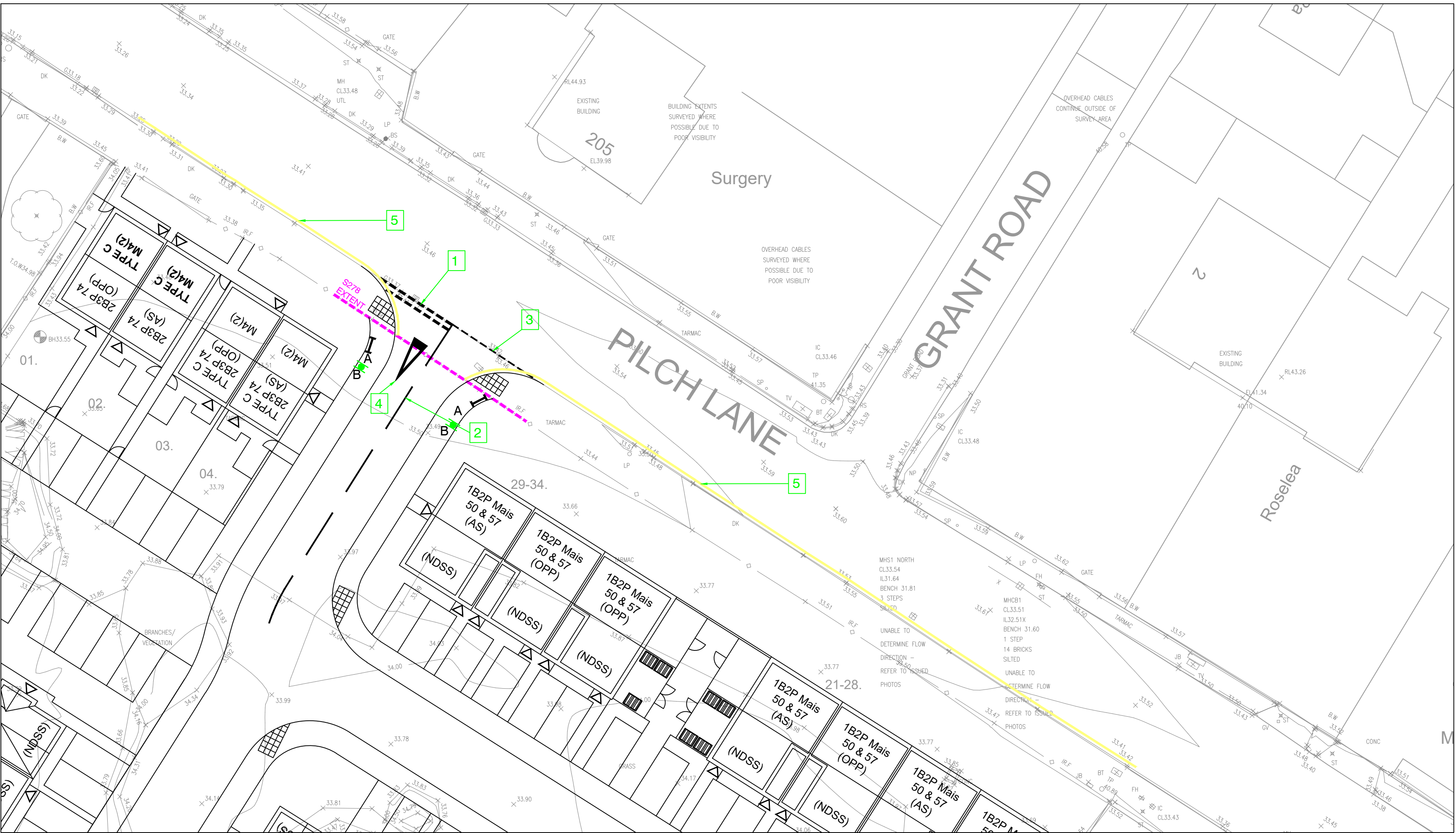
S278 Signing & Lining Layout Scale 1:250
