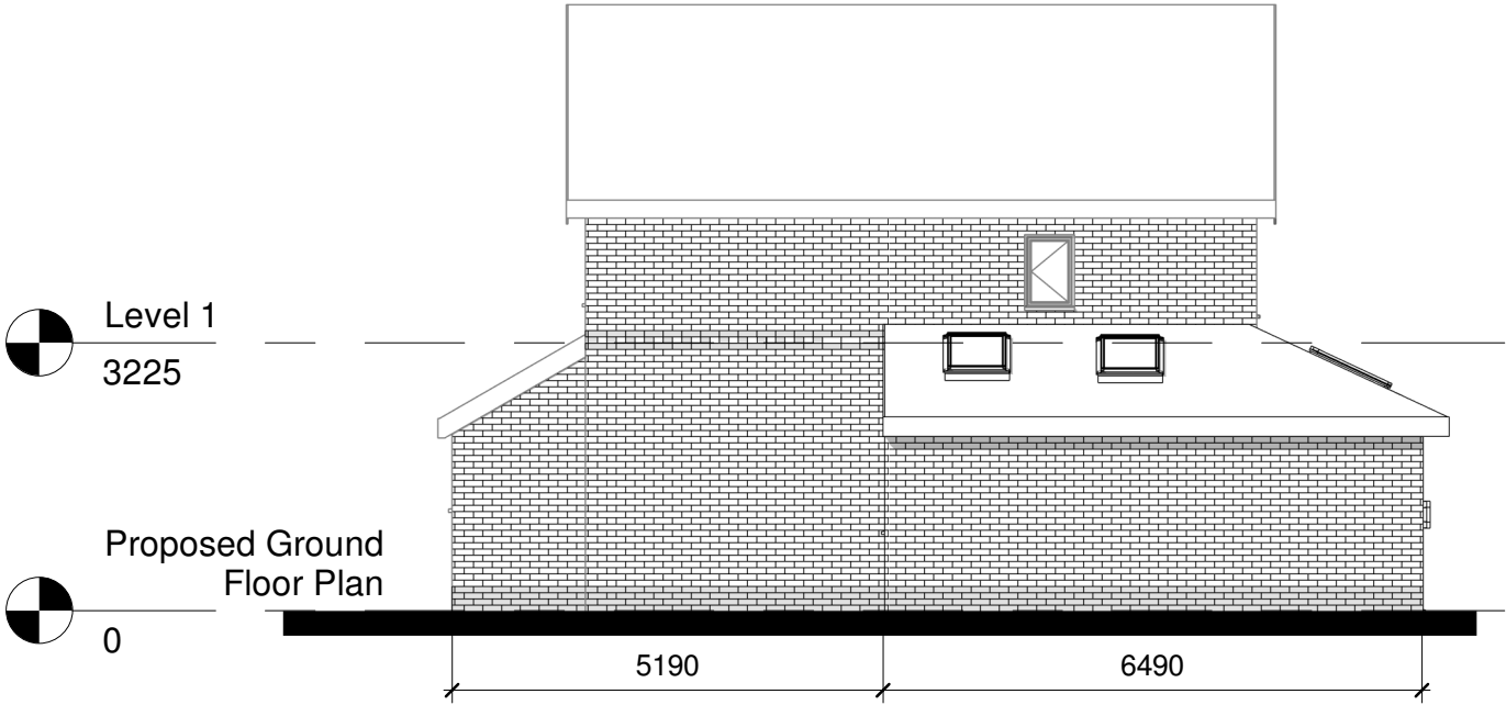
Prop. Gable Elevation 1 : 100
