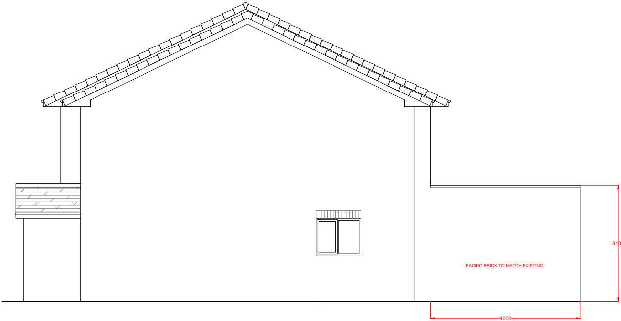
Proposed South Side Elevation 1:100
