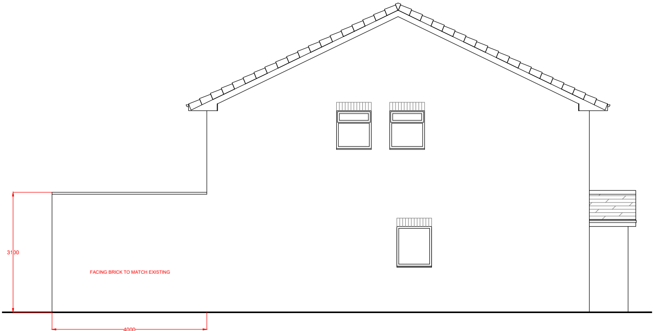
Proposed North Side Elevation 1:100
