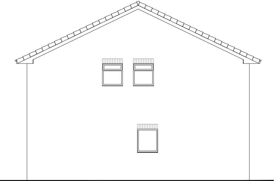
Existing North Side Elevation 1:100
