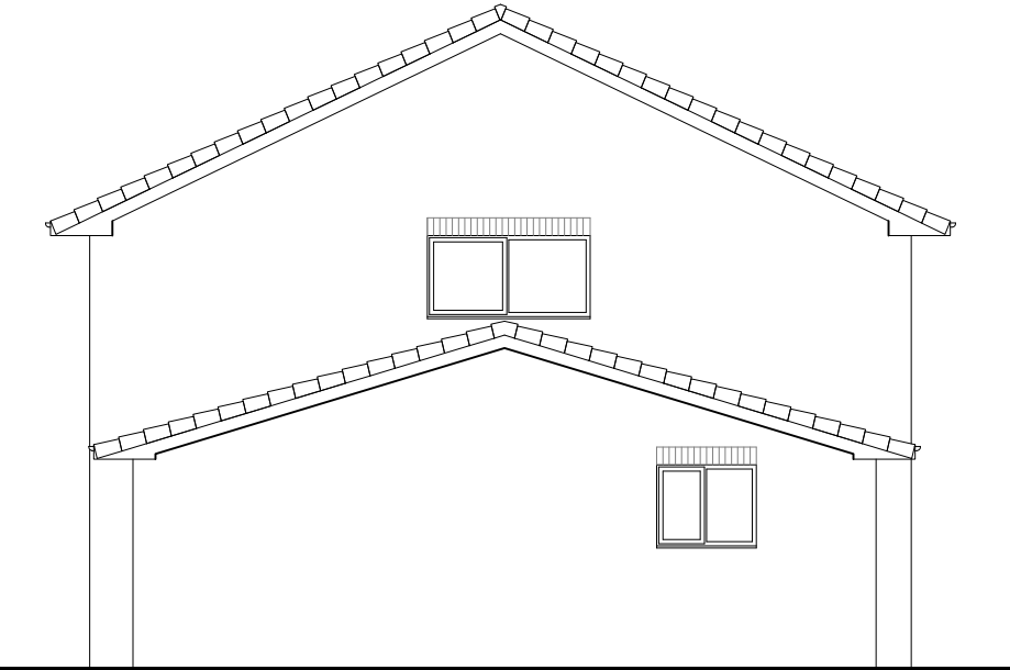
Existing South Side Elevation 1:100
