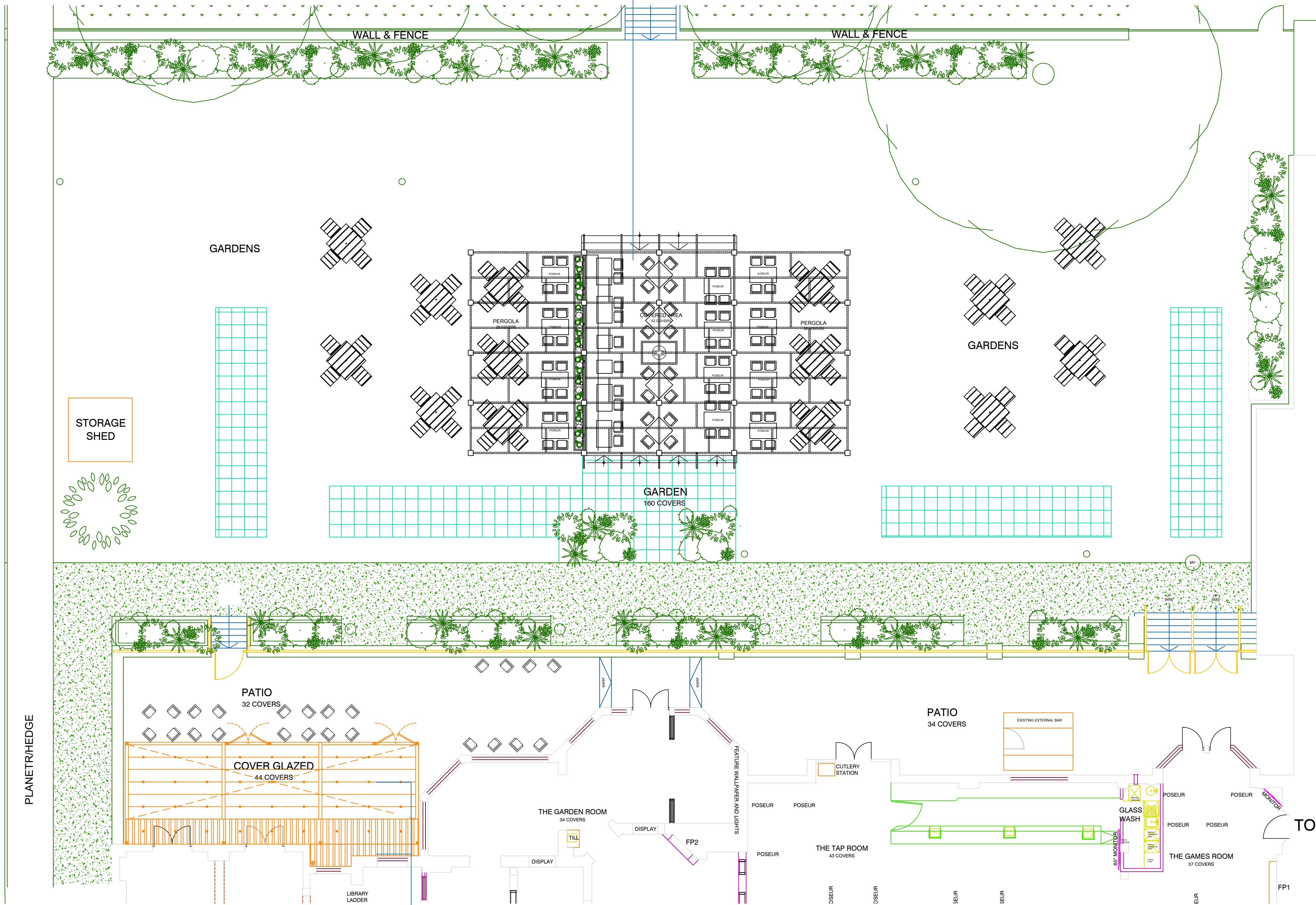
PROPOSED PLAN Scale 1:100 @ A1
