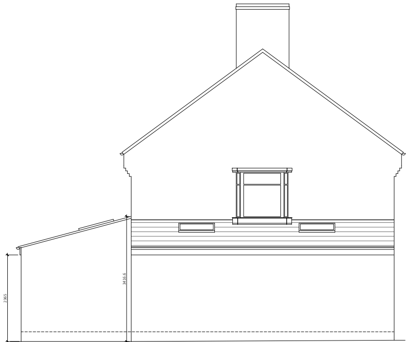
SIDE ELEVATION
