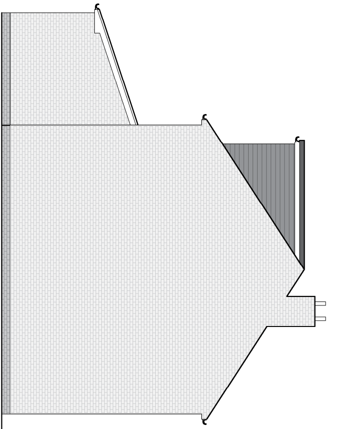
PROPOSED S DE ELEVATION (Scale 1:100) SCALE BAR - (mm) 500 1000 2000
