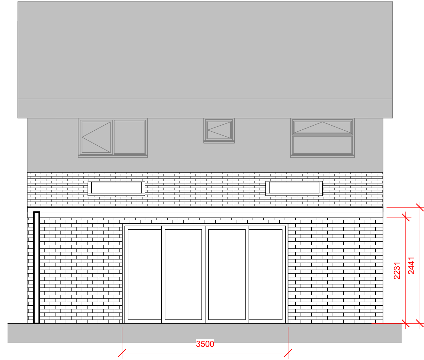
Rear Elevation 1 : 50
