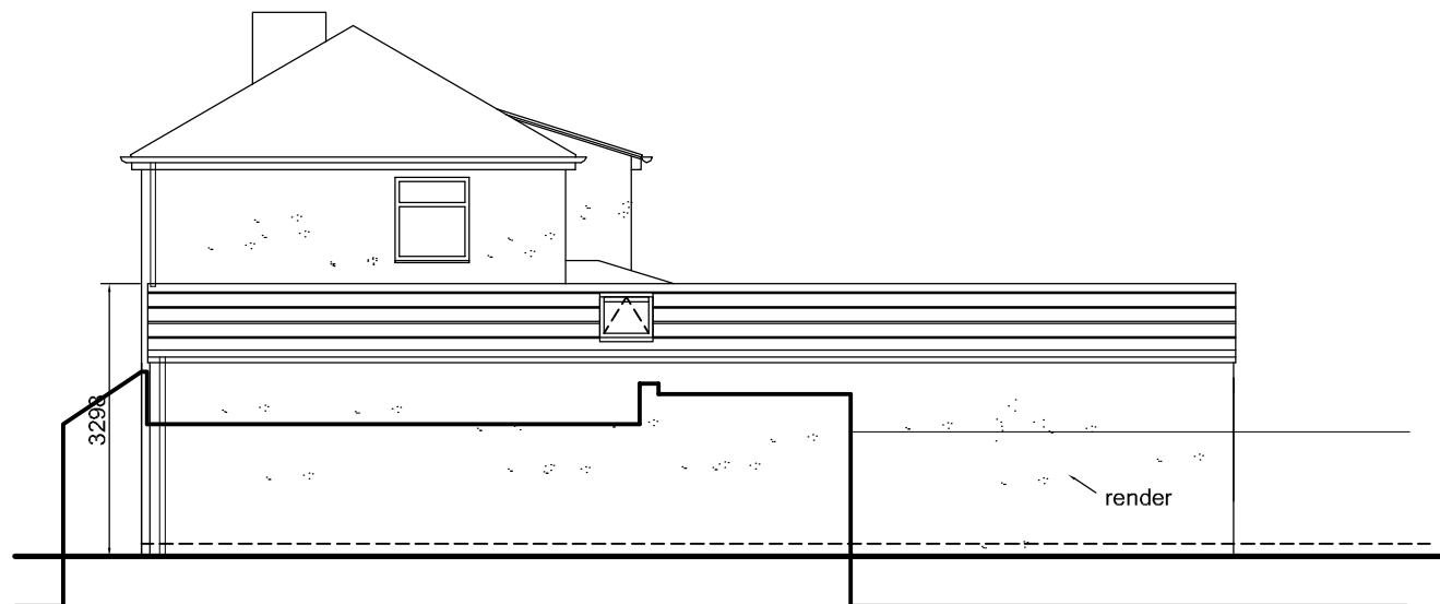
SIDE PROPOSED
