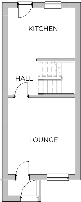
Existing Ground Floor Plan 1:100
