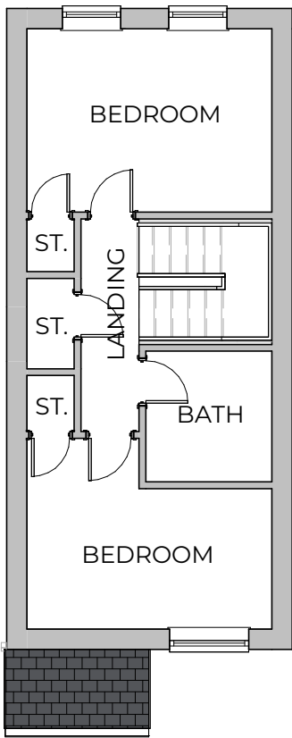
Existing First Floor Plan 1:100
