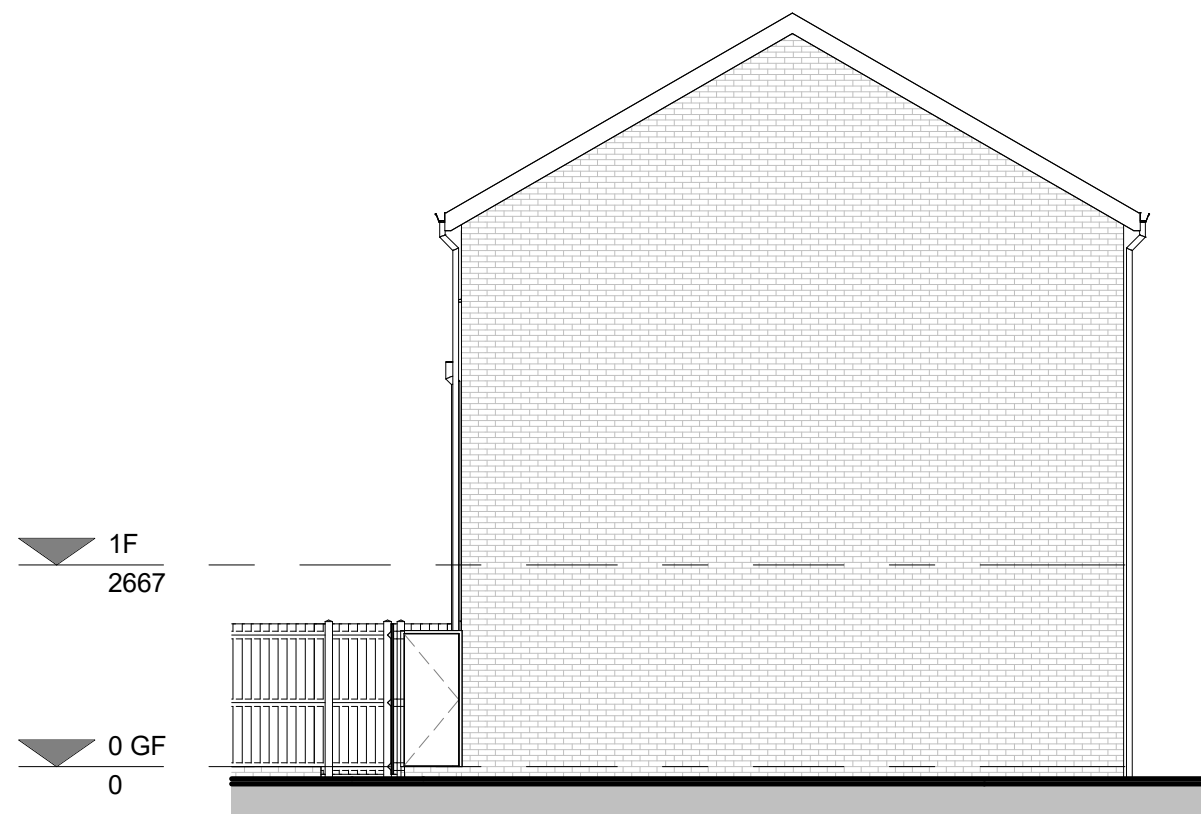
SIDE ELEVATION I
