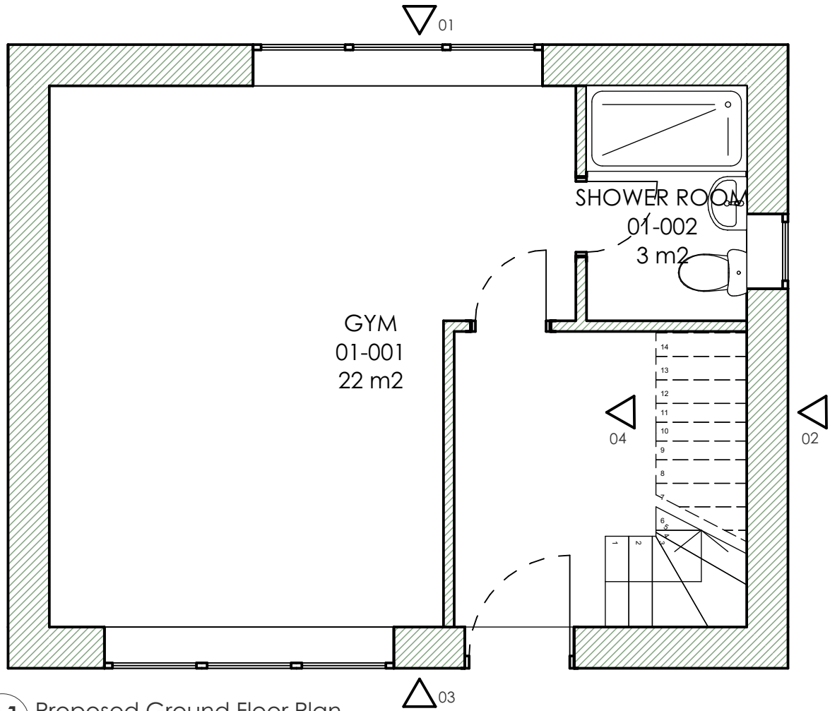
01 Proposed Ground Floor Plan 1:50
