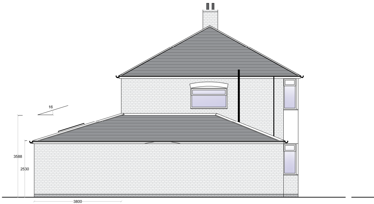
PROPOSED SIDE ELEVATION (Scale 1:100) SCALE BAR - (mm) 0 500 1000 2000
