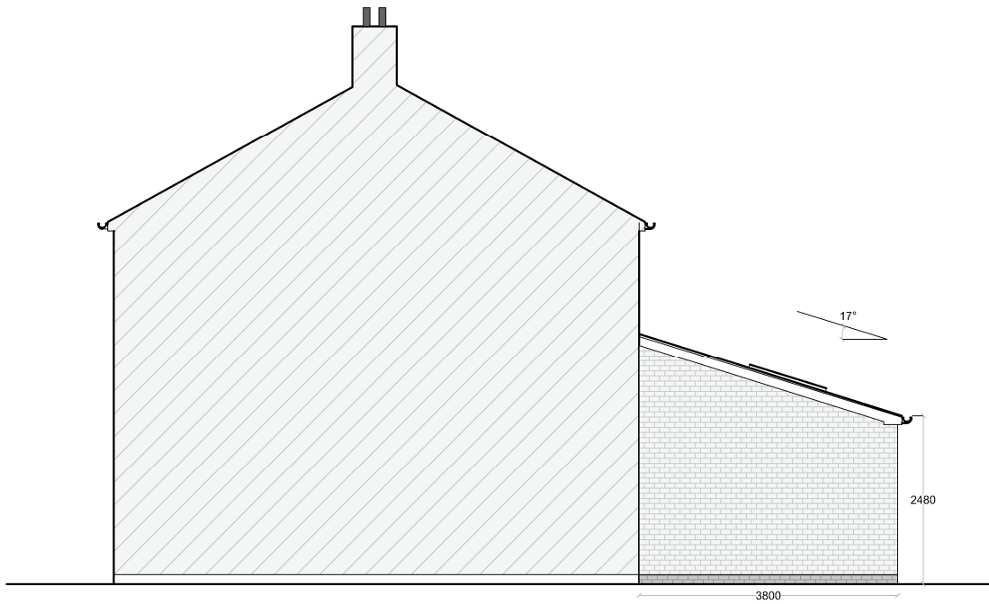
PROPOSED SIDE ELEVATION (Scale 1:100) SCALE BAR - (mm) 0 500 1000 2000
