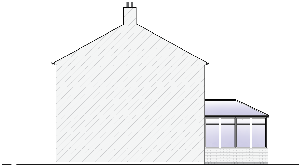
EXISTING SIDE ELEVATION (Scale 1:100) SCALE BAR - (mm) 0 500 1000 2000
